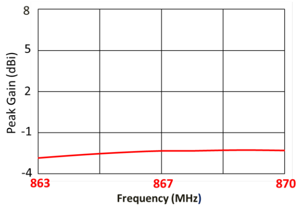
Peak Gain
