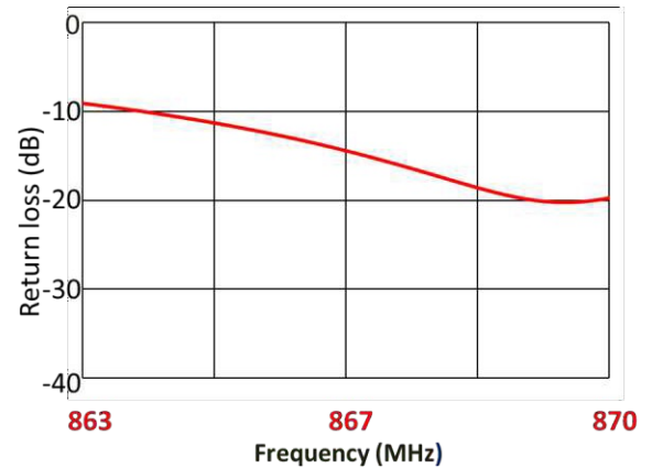
Return Loss
