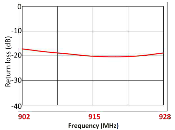
Return Loss
