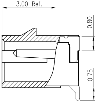
SECTION X-X
