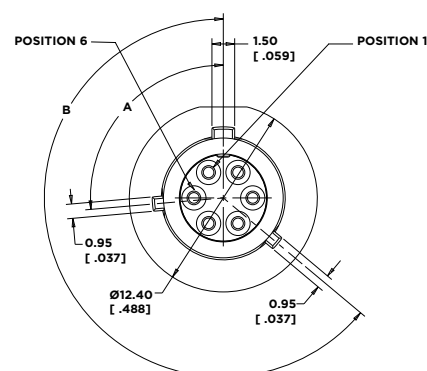
Plug Key
