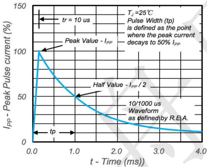
Fig.3 Pulse Waveform
