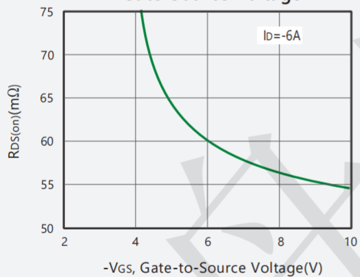
Figure 3. On-Resistance vs. Gate-Source Voltage
