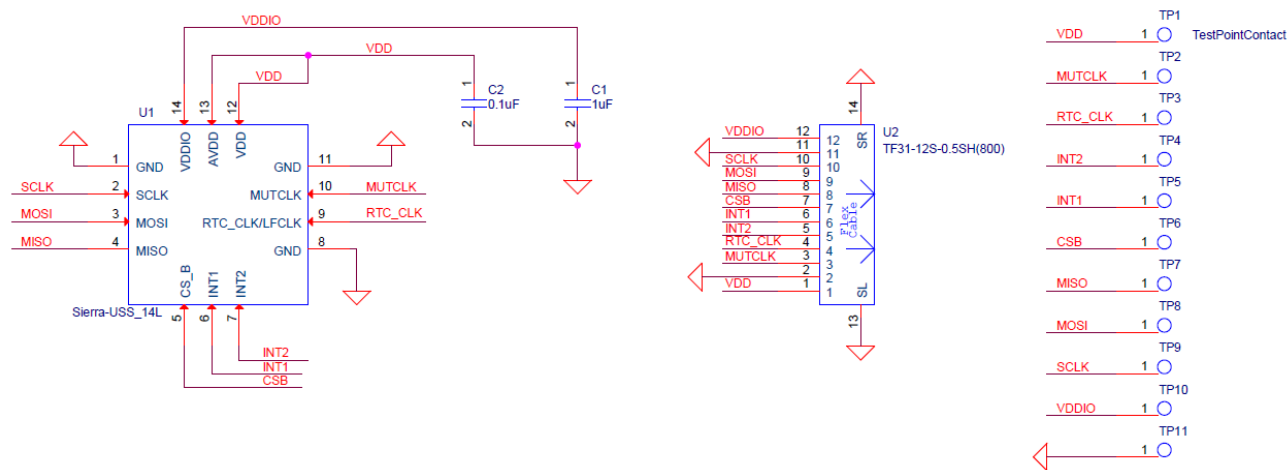
Figure 2. Schematic
