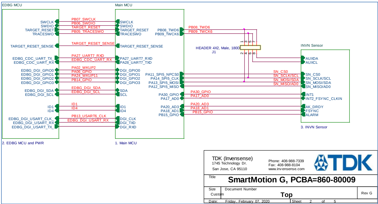
Figure 4. Hierarchy Top
