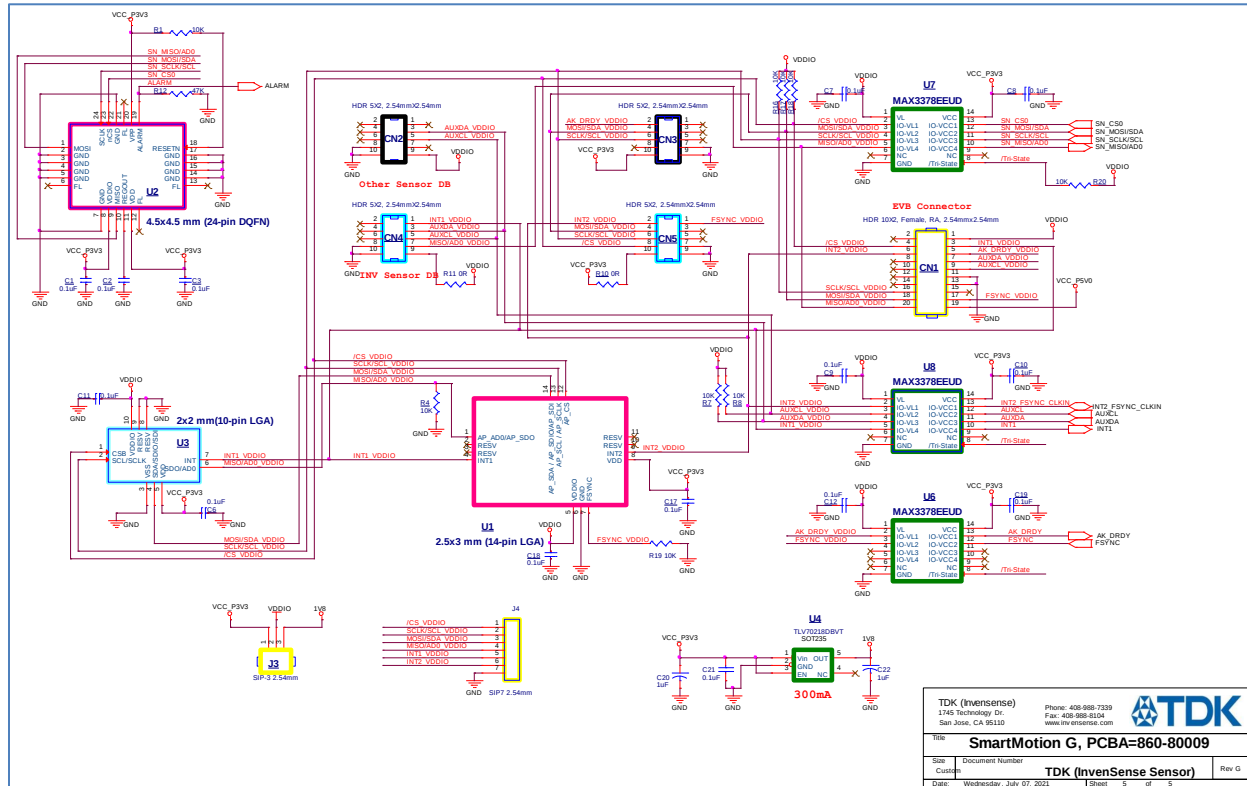
Figure 7. Sensors, DB and EVB connectors
