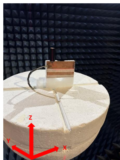
TS.16 Tested on 9x15cm Ground Plane (Longside)
