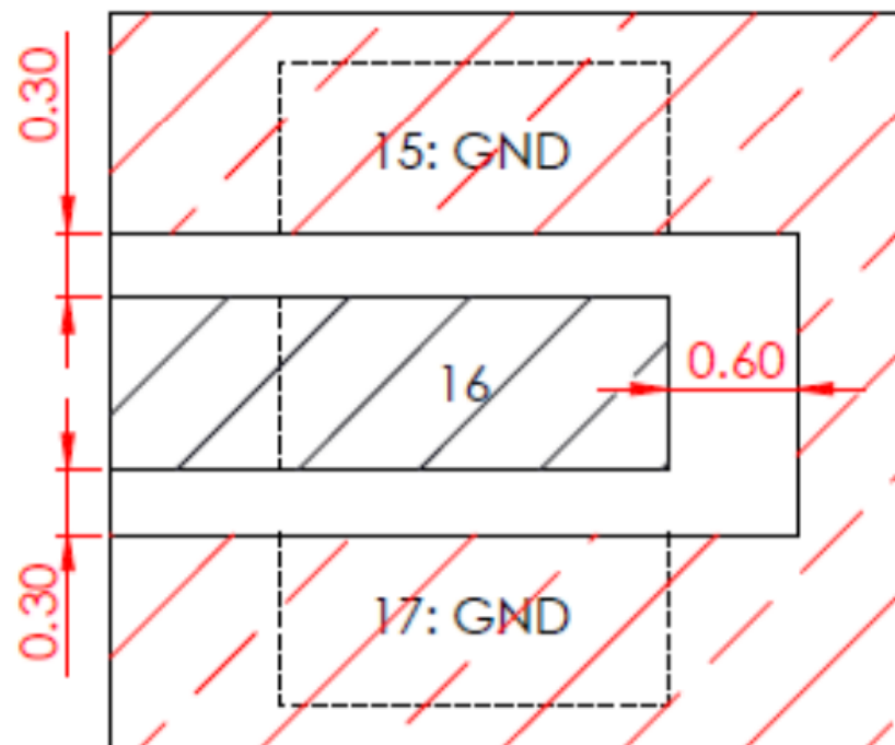
Copper Clearance for Pin 16 (RF OUT Pad) of the TFM.115A.
