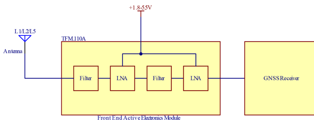
Block Diagram of integration of the TFM.110A
