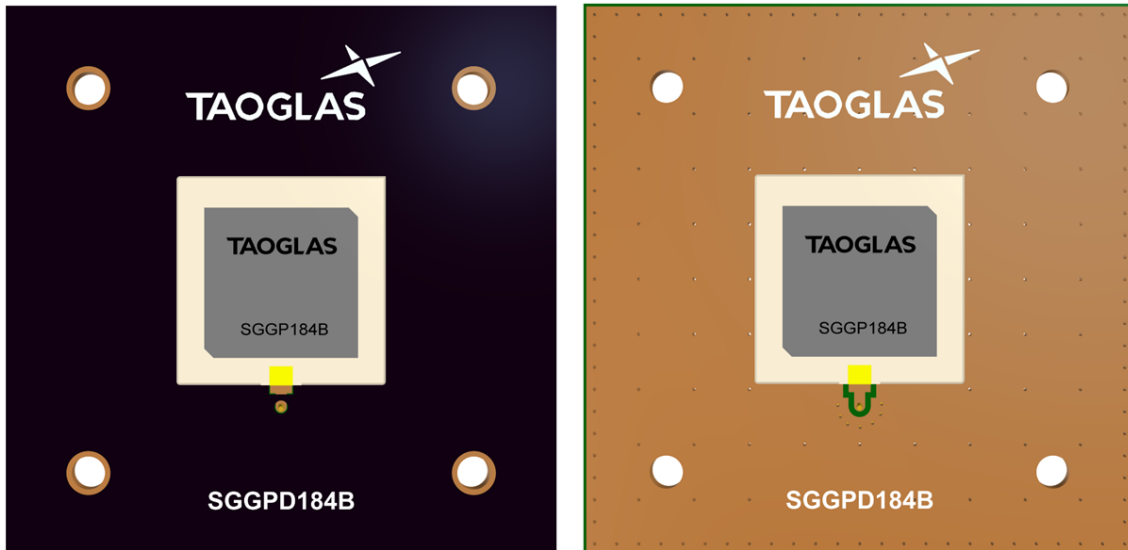
Top Side (SGGP184B placement on 50x50mm PCB reference design)
