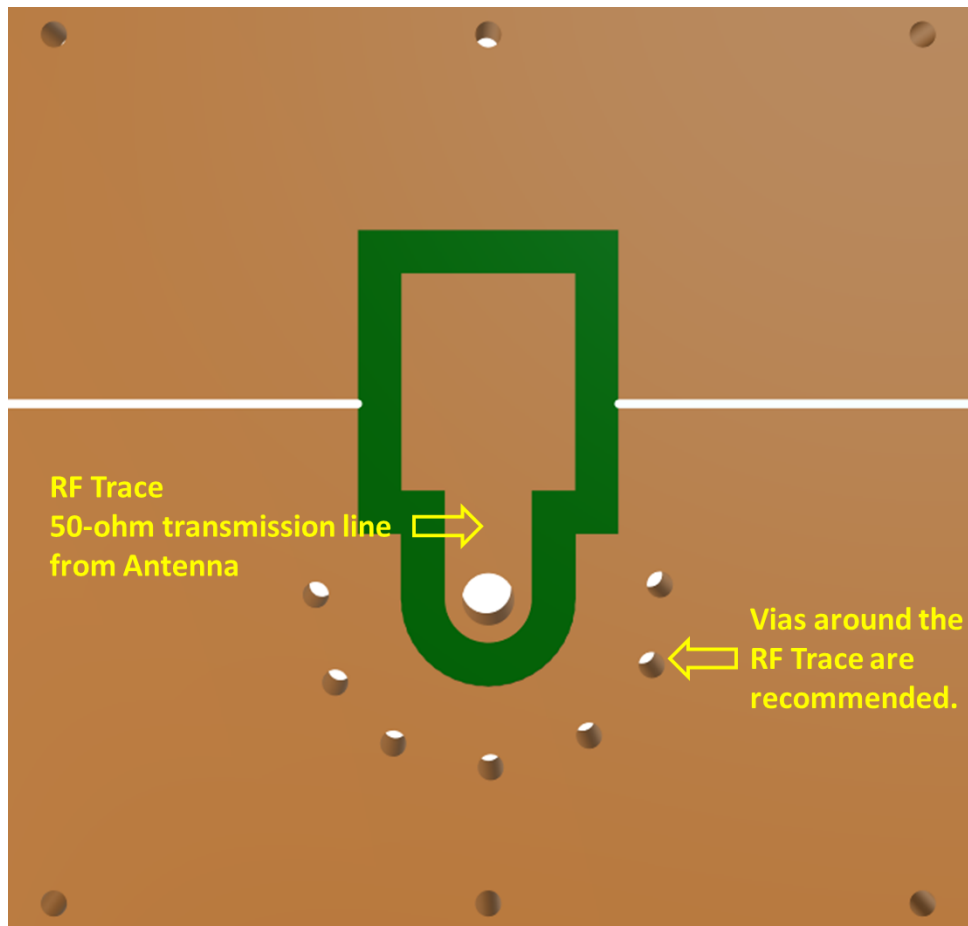
SGGP184B antenna mounted on a PCB reference design, showing transmission lines and integration notes.
