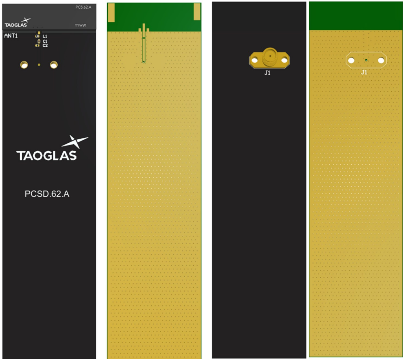
Top Side (PCS.62.A placement on 133x38mm PCB reference design)
