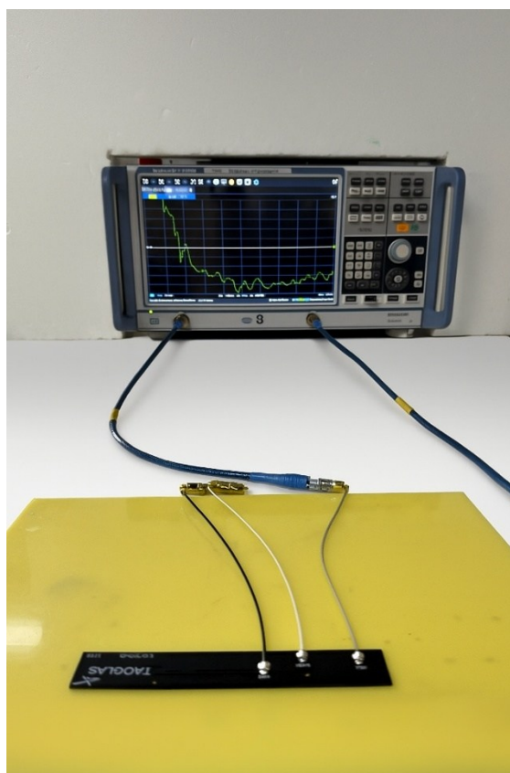
VNA Test Setup on 2mm ABS
