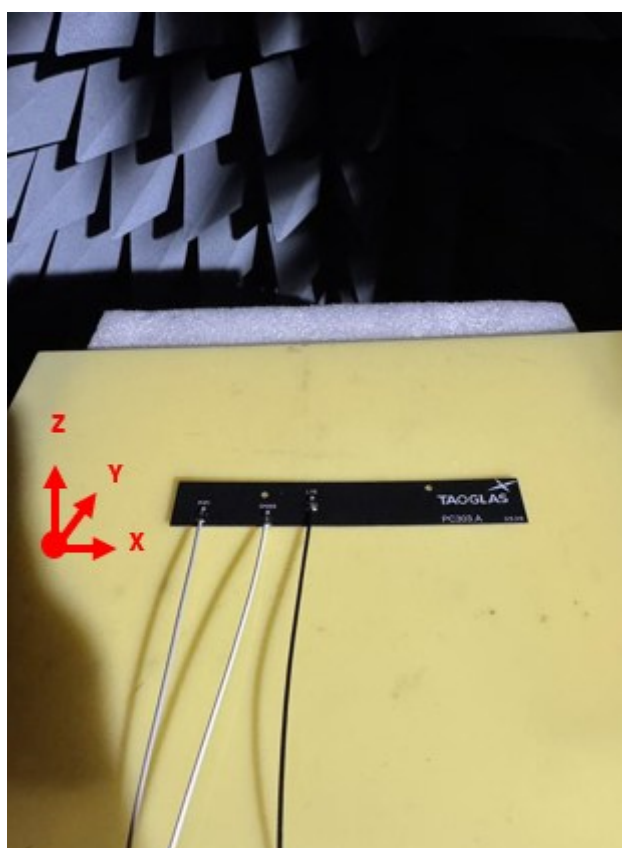
Chamber Test Setup on 2mm ABS
