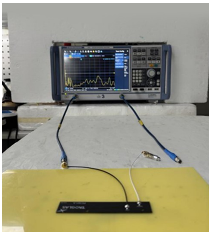
VNA Test Setup on 2mm ABS
