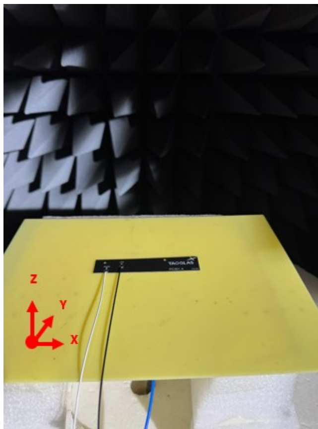
Chamber Test Setup on 2mm ABS
