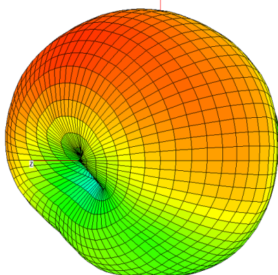
MIMO 1 – 30cmx30cm Ground Plane
