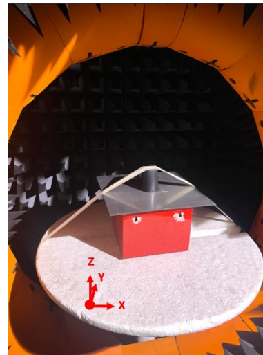
Metal Box
