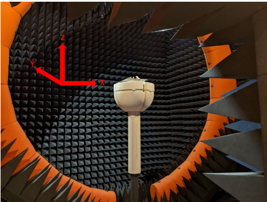
Antenna tested with underside-notch/logo centered along Y-Axis.
