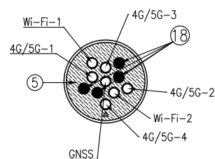
BottomThread View
