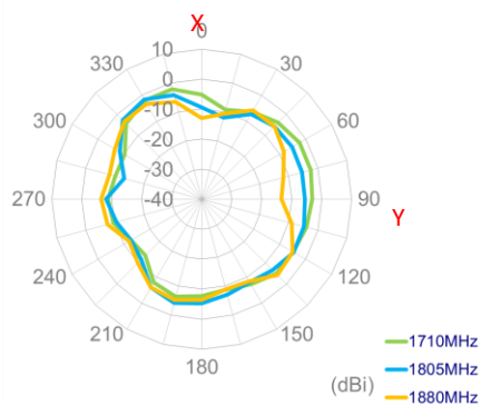
XY Plane
