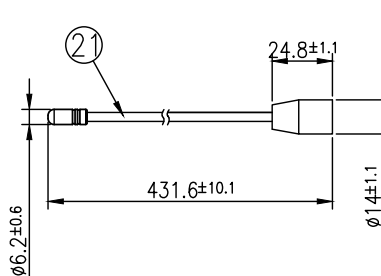
Whip Antenna-1(FW.19.M6.F): 150-174/430-520/700-900MHz Flexible Whip Antenna with M6 female connector
