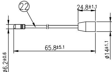
Whip Antenna-2(FW.79.M6.F): 700-900MHz Flexible Whip Antenna with M6 Female Connector
