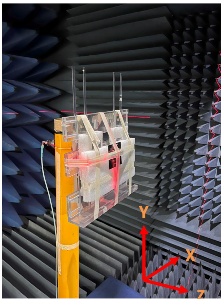
Chamber Test Set-up
