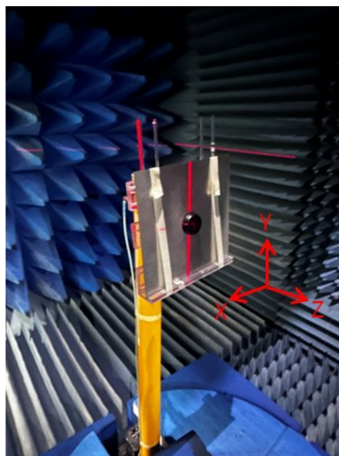
Chamber Setup on a 30x30cm Ground Plane.
