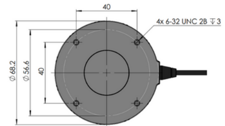
Mechanical Dimensions (mm)
