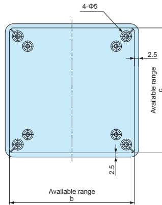
Cover (Internal)
