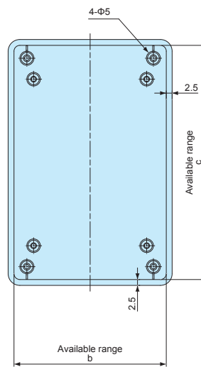
Cover (Internal)
