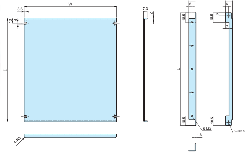
■ Mounting plate and L-bracket set.
