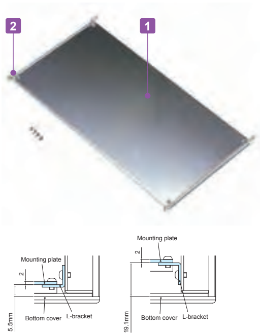
■ Mounting plate and L-bracket set.
