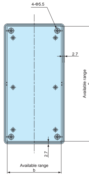
Cover (Internal)
