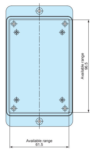
Flanged base (Internal)
