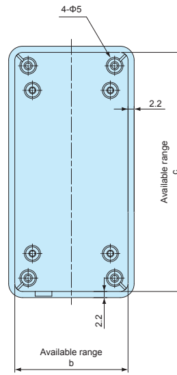
Cover (Internal)
