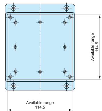
Flanged base (Internal)
