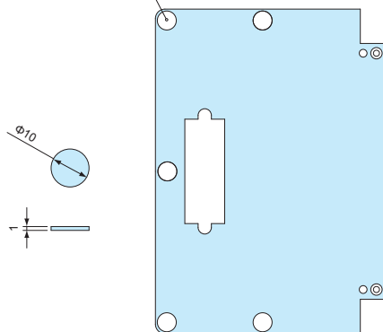
Back side of open / closing panel
