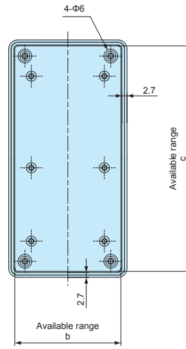
Cover (Internal)
