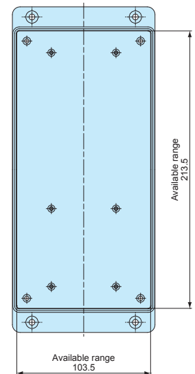
Flanged base (Internal)
