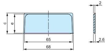
Panel dimensions
