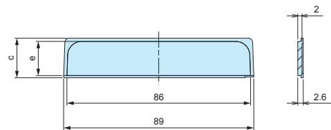
Panel dimensions
