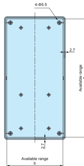
Cover (Internal)
