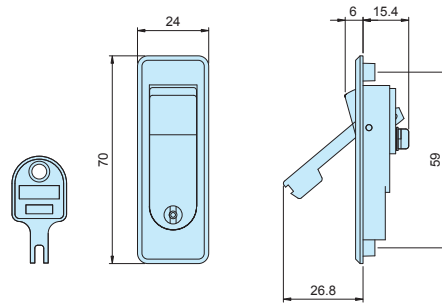
Key lock type
