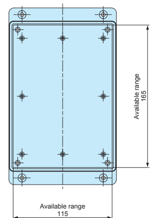
Flanged base (Internal)
