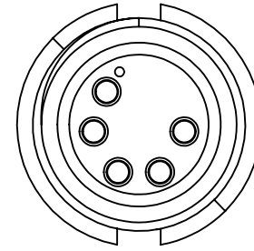
W3280-5PG-P-5XX WIRING VIEW
