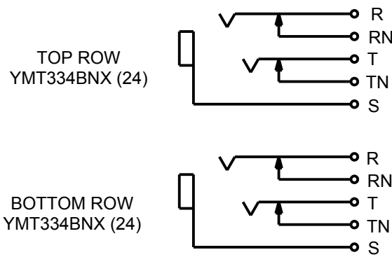
MT48FNX SCHEMATIC
