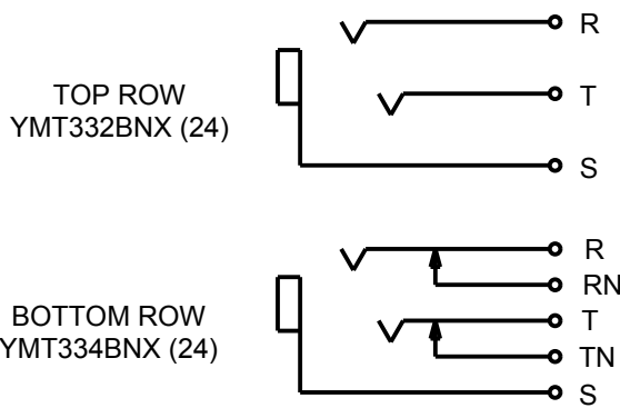
MT48HNX SCHEMATIC
