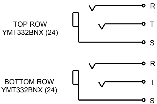
MT48NNX SCHEMATIC
