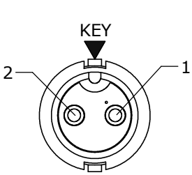
FACE VIEW 6380-2PG-5XX
