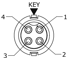
FACE VIEW 6380-4PG-5XX
