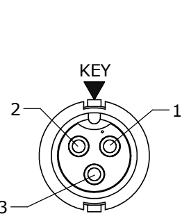
FACE VIEW 6380-3PG-5XX
