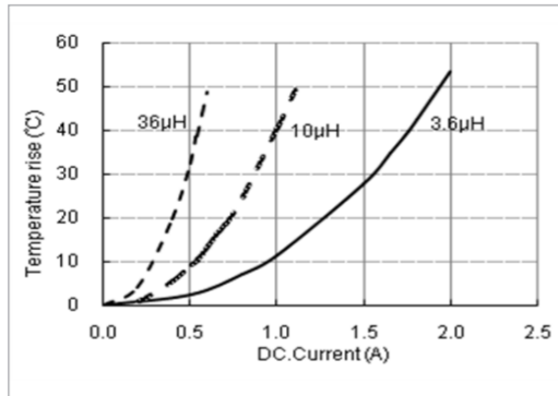
SWPA4018S Series Temperature vs. DC Current Characteristics
