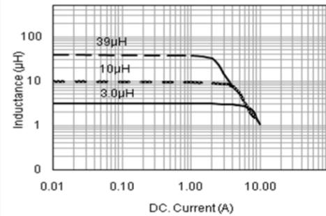
Inductance vs. DC Current Characteristics
