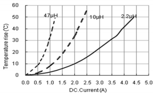
SWPA6045S Series Temperature vs. DC Current Characteristics
