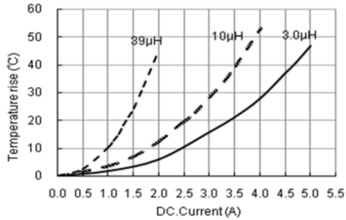
SWPA8065S Series Temperature vs. DC Current Characteristics
