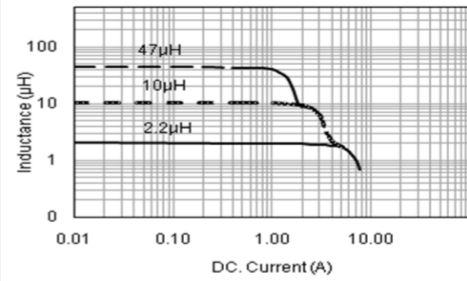
Inductance vs. DC Current Characteristics
