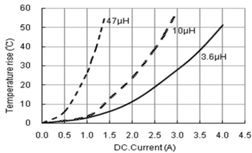
SWPA8040S Series Temperature vs. DC Current Characteristics
