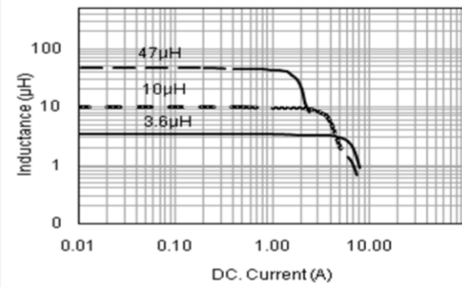
Inductance vs. DC Current Characteristics
