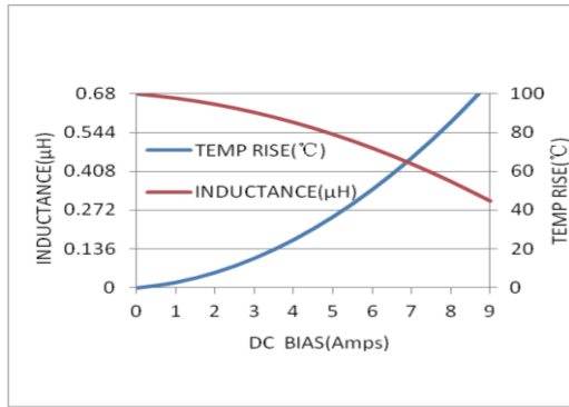
MWSA0412S-R68MT
