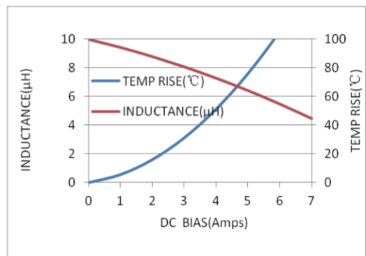
MWSA0624S-100MT
