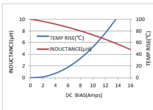
MWSA1204S-100MT
