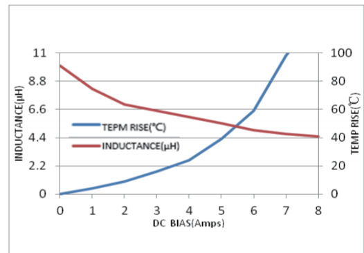
MWSA0402S-100MT
