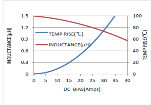
MWSA1204S-1R5MT
