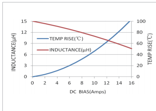
MWSA1205S-150MT
