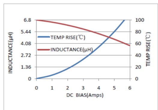
MWSA0618S-6R8MT
