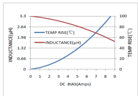
MWSA0618S-3R3MT
