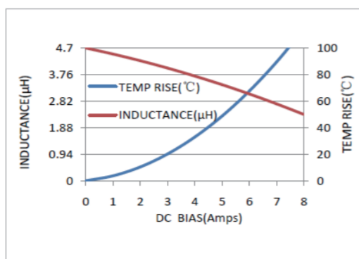
MWSA0618S-4R7MT
