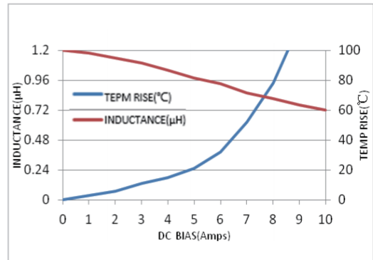
MWSA0402S-1R2MT
