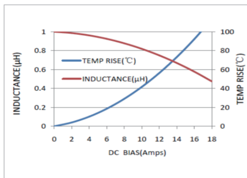
MWSA0618S-1R0MT
