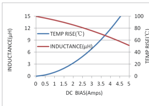
MWSA0624S-150MT
