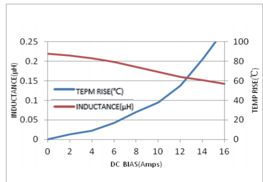
MWSA0402S-R22MT
