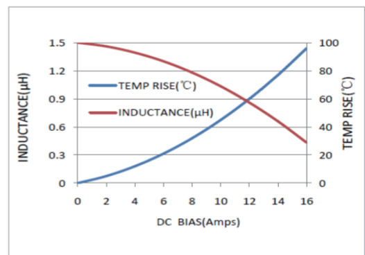
MWSA0618S-1R5MT
