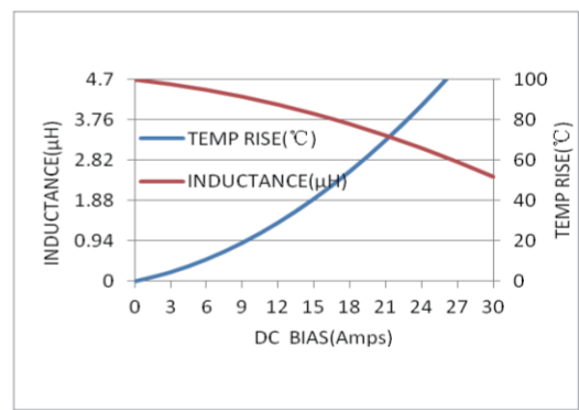
MWSA0624S-4R7MT
