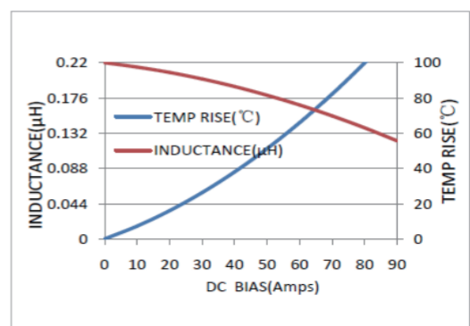
MWSA1004S-R22MT
