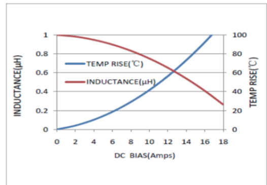
MWSA0503S-1R0MT
