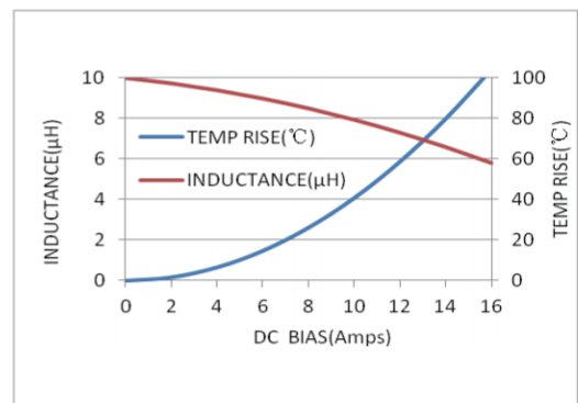
MWSA1205S-100MT
