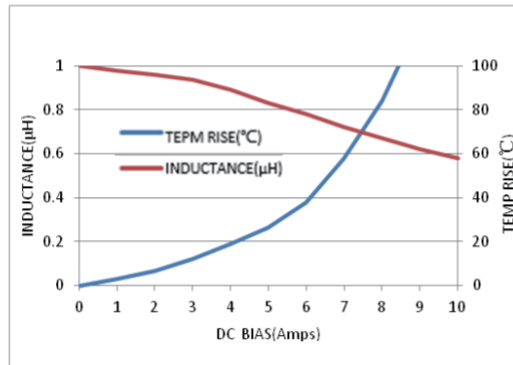
MWSA0402S-1R0MT
