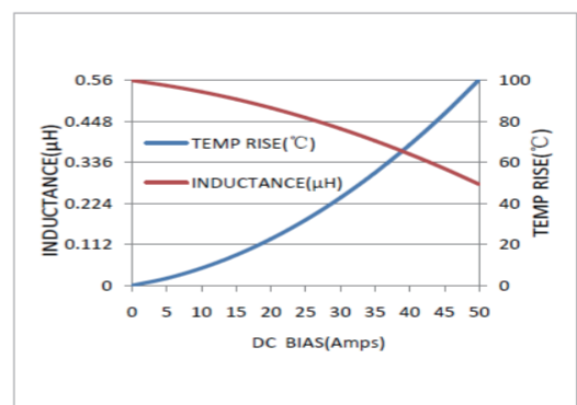
MWSA1004S-R56MT
