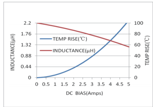
MWSA0412S-2R2MT
