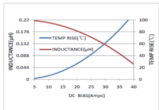
MWSA0618S-R22MT
