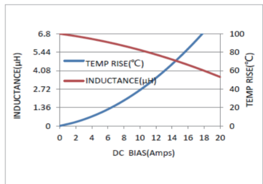
MWSA1204S-6R8MT
