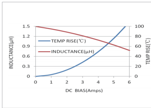
MWSA0412S-1R5MT
