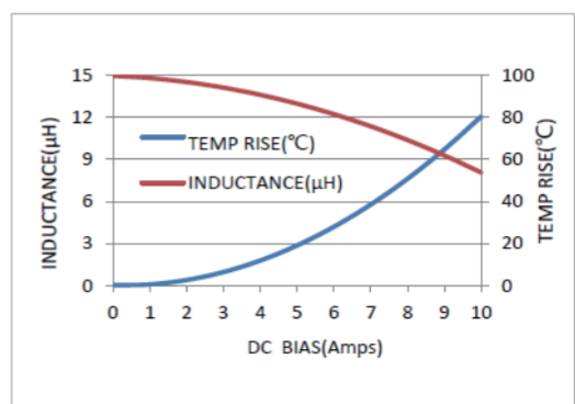
MWSA1204S-150MT
