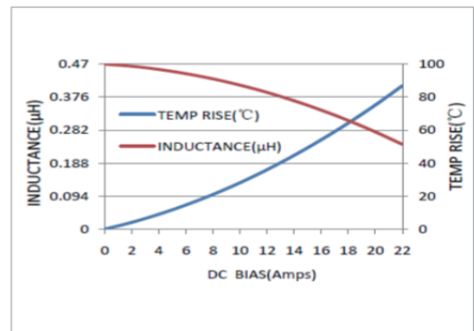
MWSA0503S-R47MT
