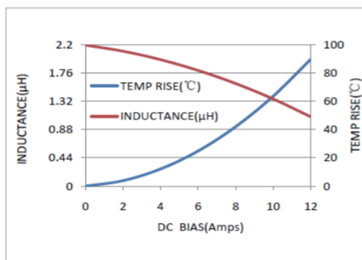
MWSA0618S-2R2MT
