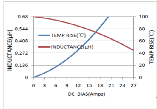
MWSA0618S-R68MT
