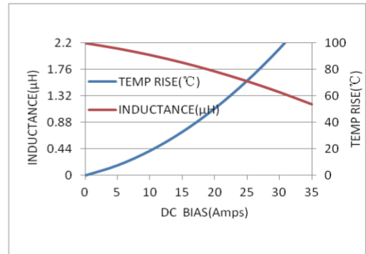
MWSA1205S-2R2MT
