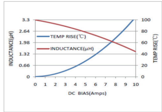
MWSA0503S-3R3MT
