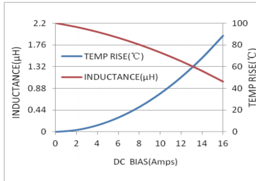
MWSA0603S-2R2MT
