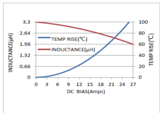
MWSA1204S-3R3MT
