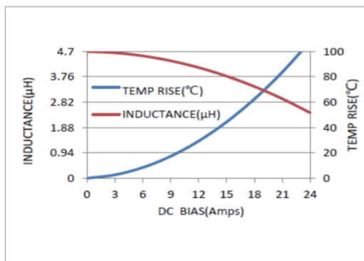
MWSA1204S-4R7MT
