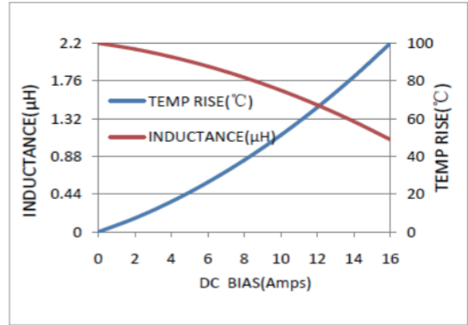
MWSA0624S-2R2MT
