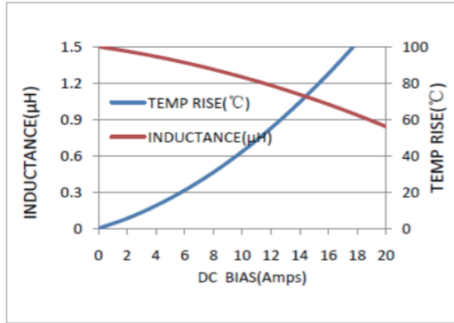
MWSA0624S-1R5MT
