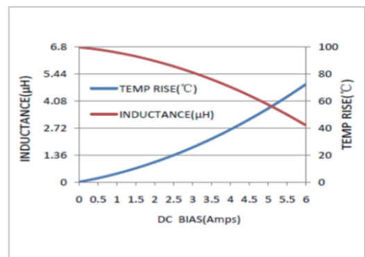
MWSA0503S-6R8MT
