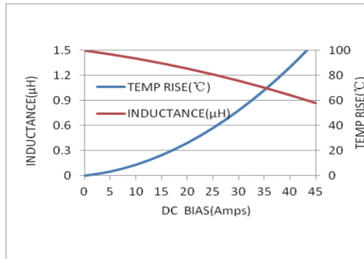
MWSA1205S-1R5MT
