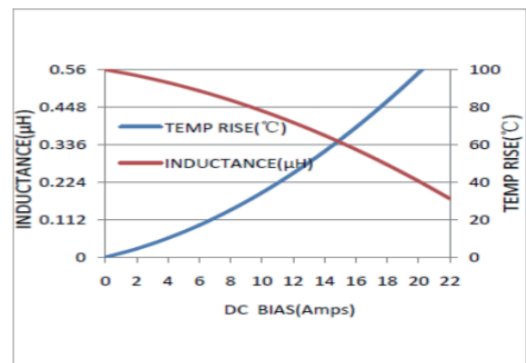
MWSA0518S-R56MT
