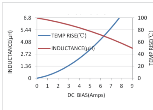
MWSA0624S-6R8MT
