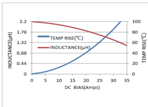
MWSA1204S-2R2MT
