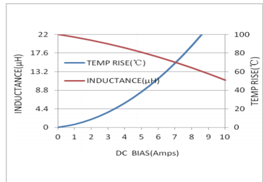
MWSA1205S-220MT
