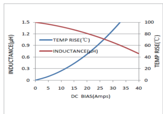
MWSA1004S-1R5MT
