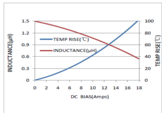
MWSA0503S-1R5MT
