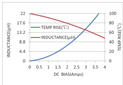
MWSA0624S-220MT
