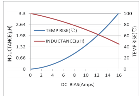
MWSA0603S-3R3MT
