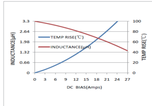
MWSA1004S-3R3MT
