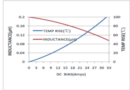
MWSA0503S-R20MT
