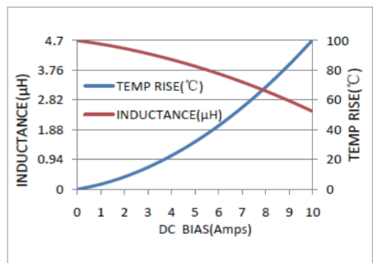
MWSA0624S-4R7MT
