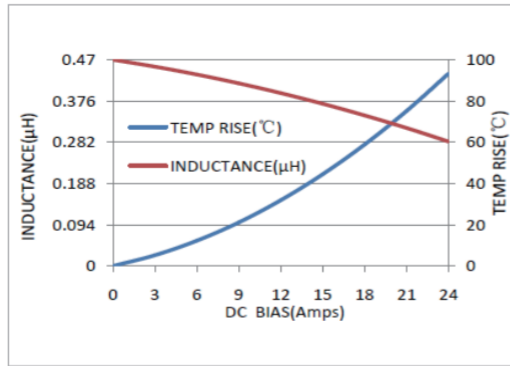
MWSA0618S-R47MT
