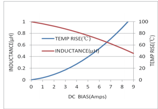
MWSA0412S-1R0MT
