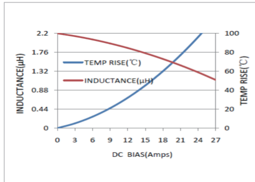
MWSA1004S-2R2MT
