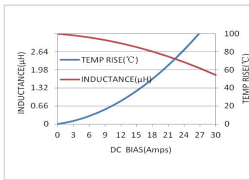
MWSA1205S-3R3MT
