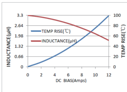
MWSA0624S-3R3MT
