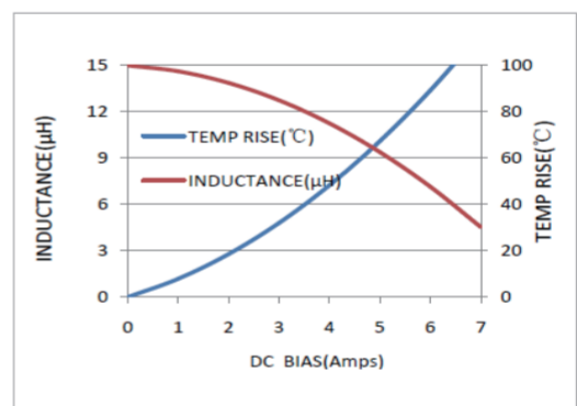
MWSA0603S-150MT
