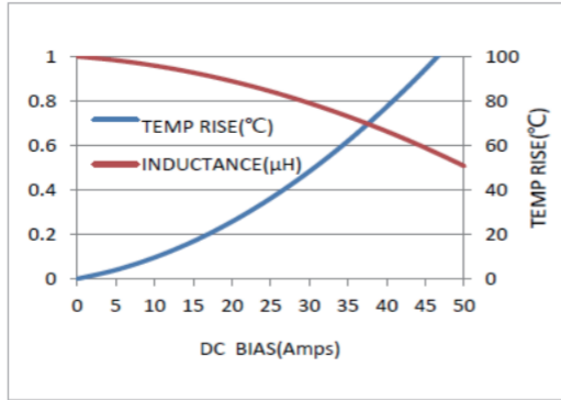
MWSA1204S-1R0MT
