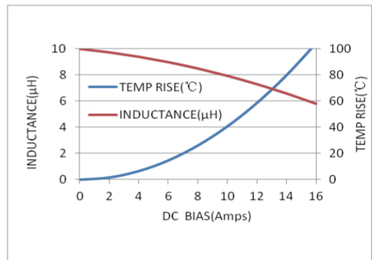
MWSA1205S-100MT
