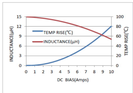
MWSA1204S-150MT
