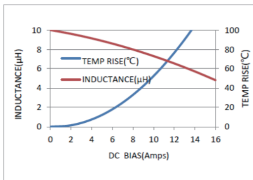
MWSA1204S-100MT
