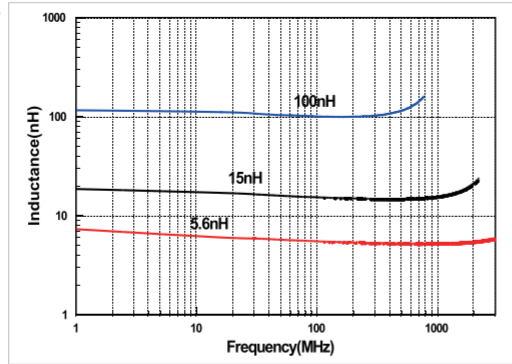
Inductance vs. Frequency Characteristics ASDCL1005-A01 TYPE
