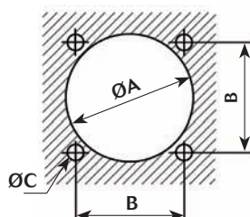
Type 0 square flange receptacle
