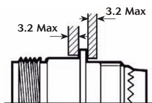
Type 0 square flange receptacle
