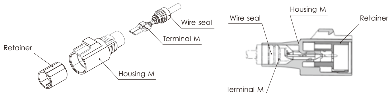
Connector M
