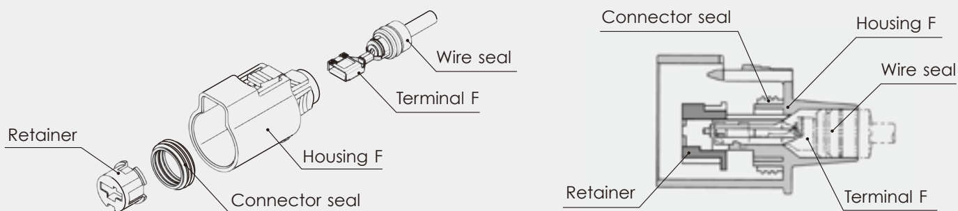
Connector F
