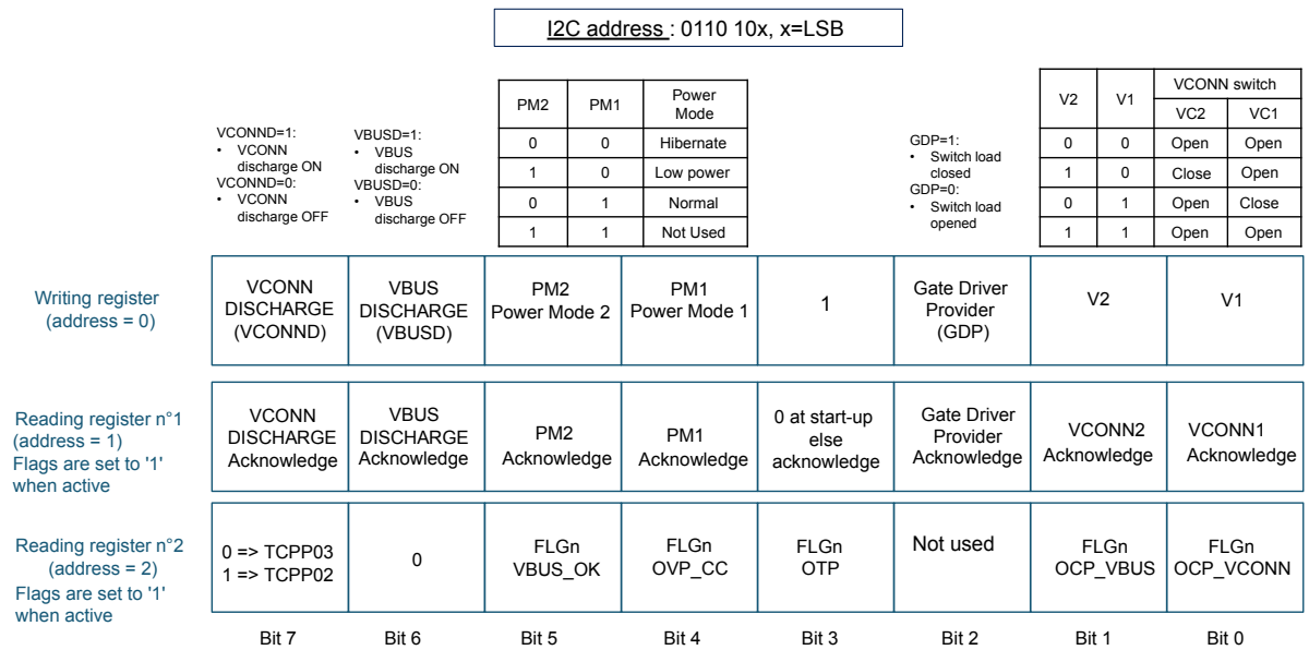
Figure 7. I2C registers
