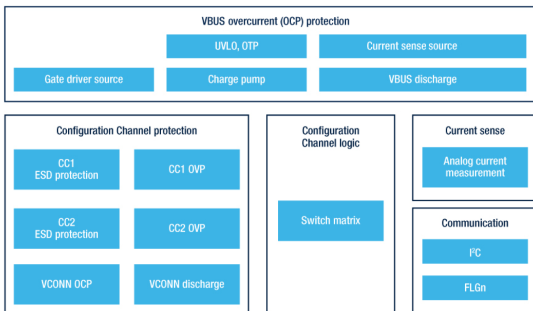
Figure 2. TCPP02-M18 functional block diagram
