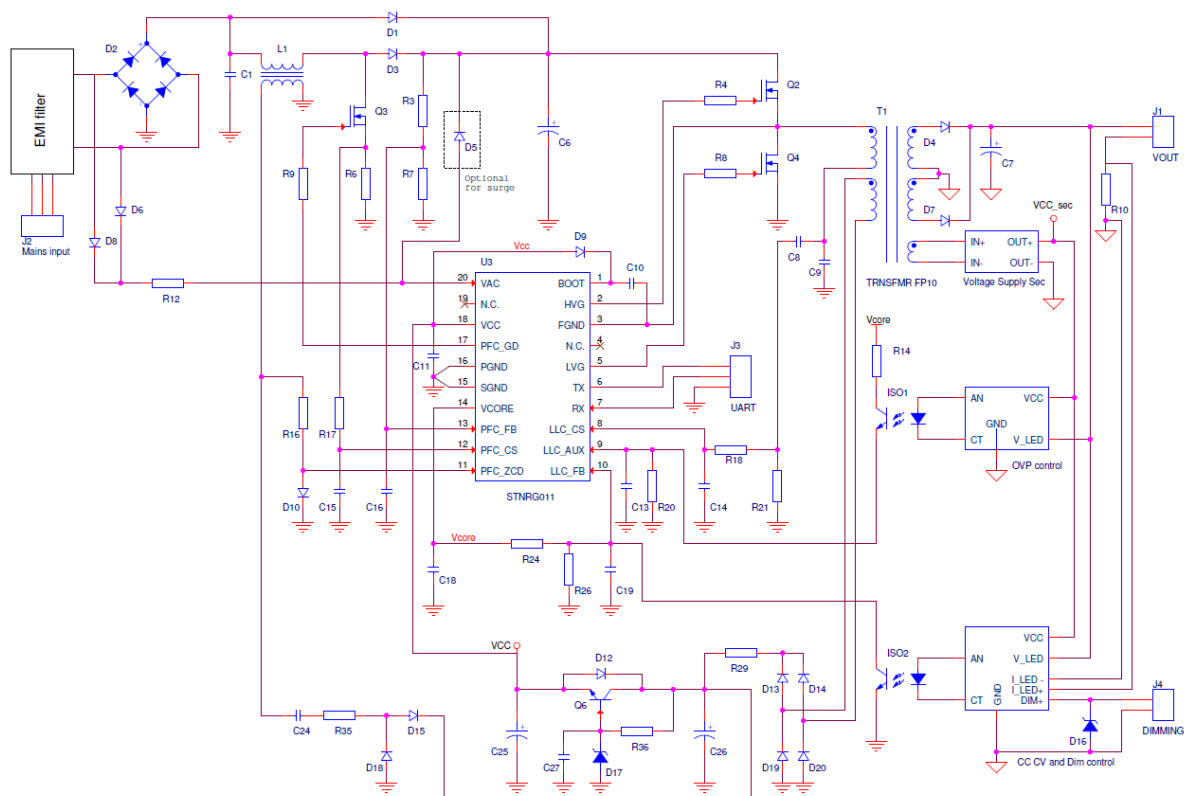
Figure 5. Typical application schematic (part 1)
