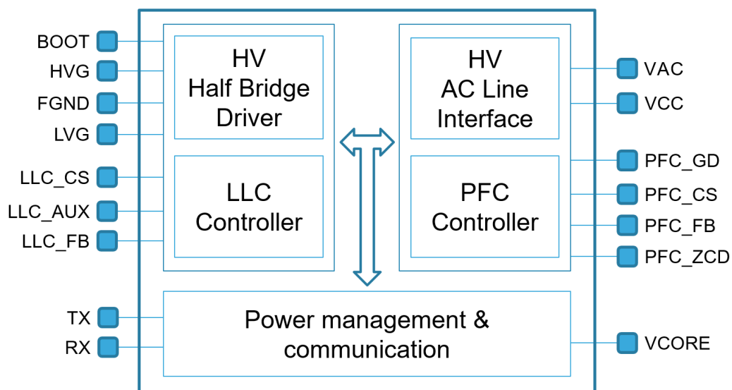
Figure 1. Block Diagram
