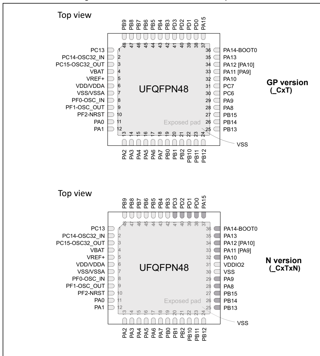
Figure 10. STM32G0B1CxU UFQFPN48 pinout
