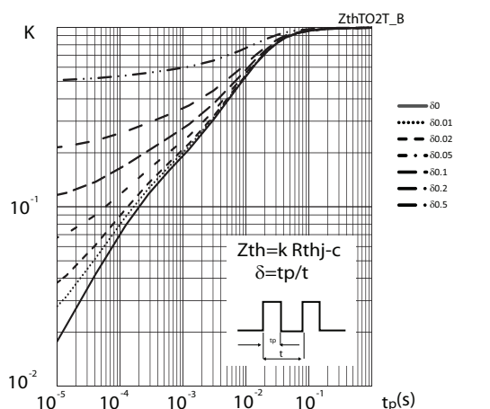
Figure 17. Thermal impedance for TO-220FP
