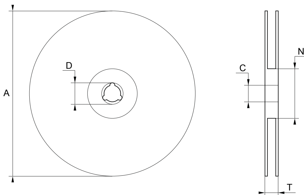
Figure 56. Reel outline
