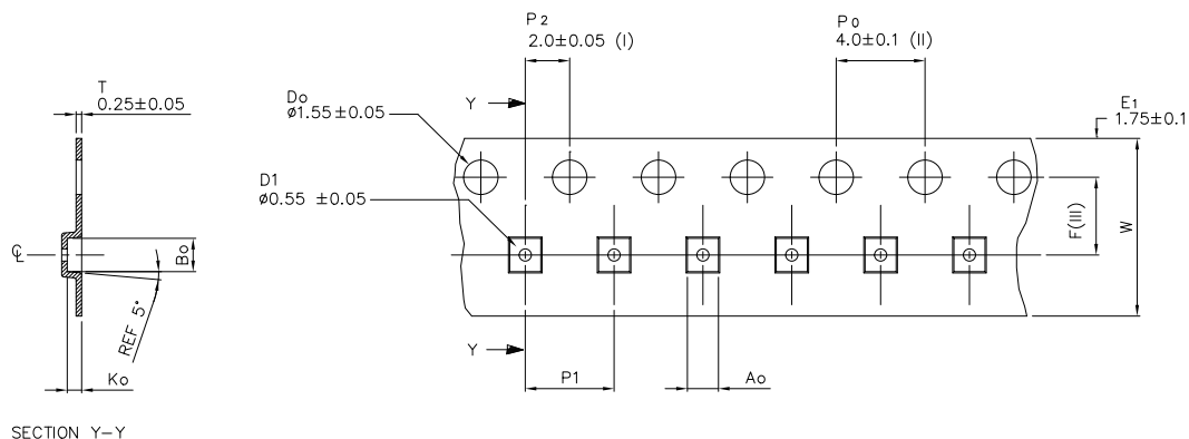
Figure 54. DFN6 tape
