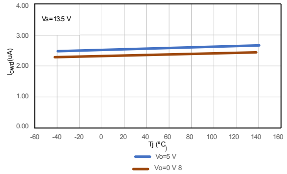
Figure 27. I cwD vs T j
