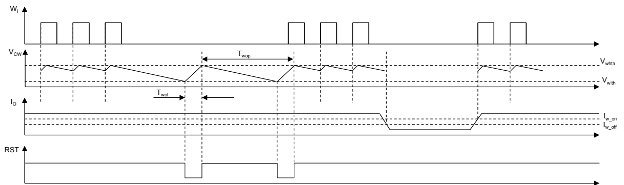
Figure 38. Watchdog timing diagram
