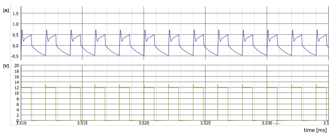
Figure 13. Simulation with appropriate masking time (330 ns)
