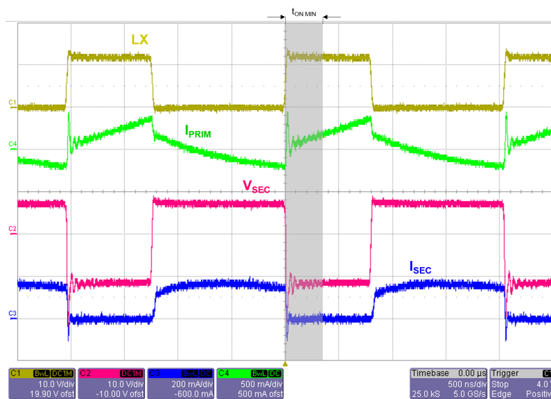
Figure 14. Remaining oscillations filtered by the masking time and RC snubber circuit V_{IN} = 12\text{ V} , N = 1.58 , I_{OUTiso} = 100\text{ mA}
