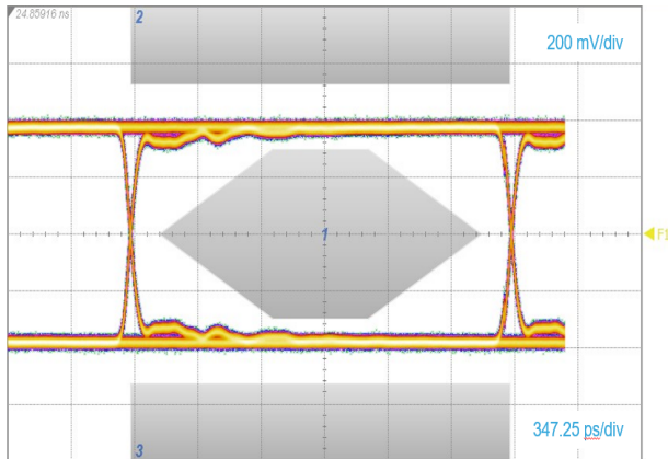
Figure 14. USB 2.0 High Speed 480 Mbps eye diagram, Template 1, without ECMFx-40A100Nx
