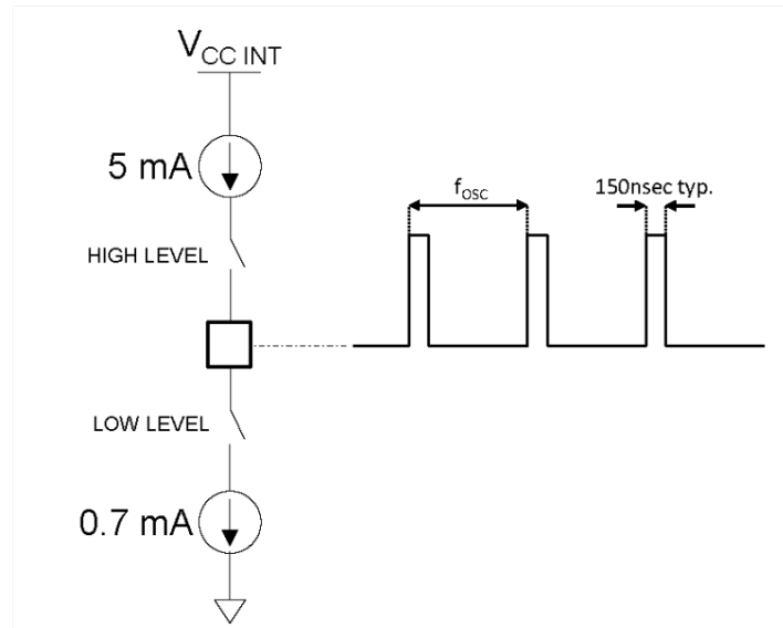
Figure 39. A6986I synchronization driving capability
