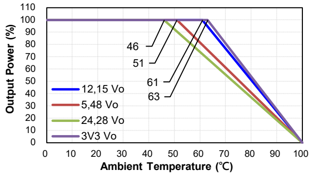
CQB150W-110S CMFC(D) Derating Curve with Heat Sink FLB254 (Vin=110V)
