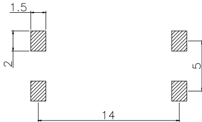
PCB.WELDING DRAWING
