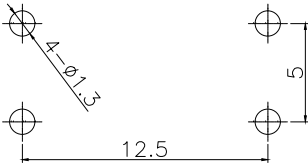
PCB.WELDING DRAWING
