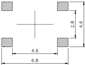
PCB.WELDING DRAWING
