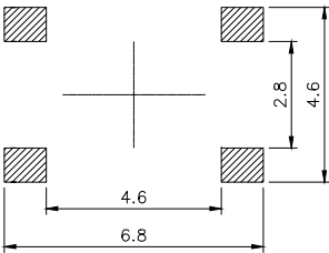
PCB.WELDING DRAWING
