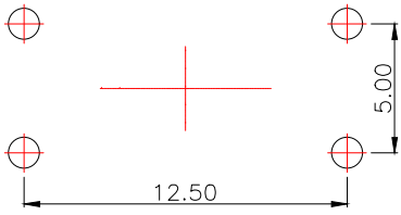
PCB.WELDING DRAWING
