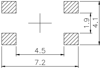
PCB.WELDING DRAWING
